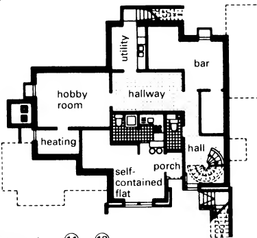
10 Basement → 11 - 13
